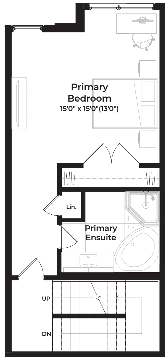
SECOND FLOOR
