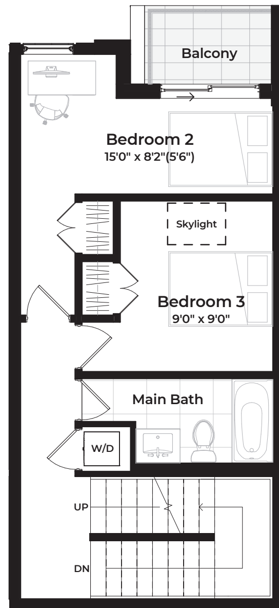
THIRD FLOOR
